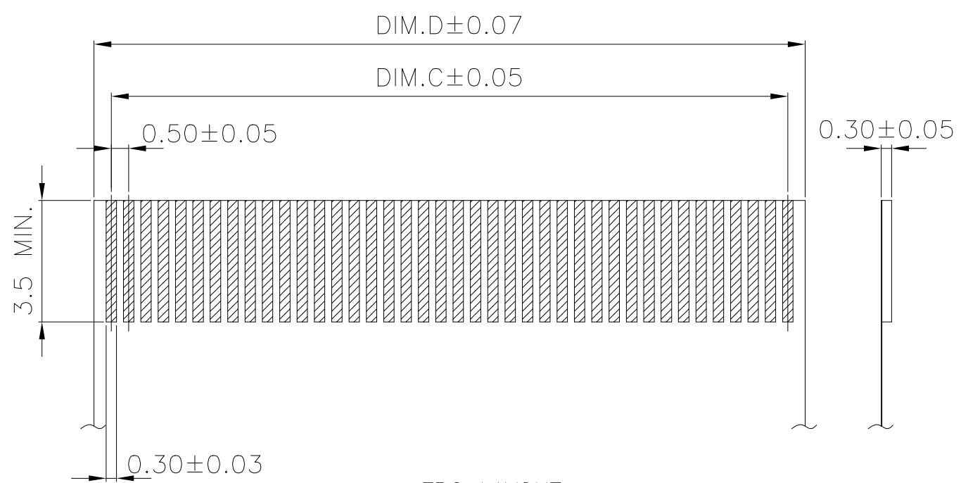
FPC LAYOUT
