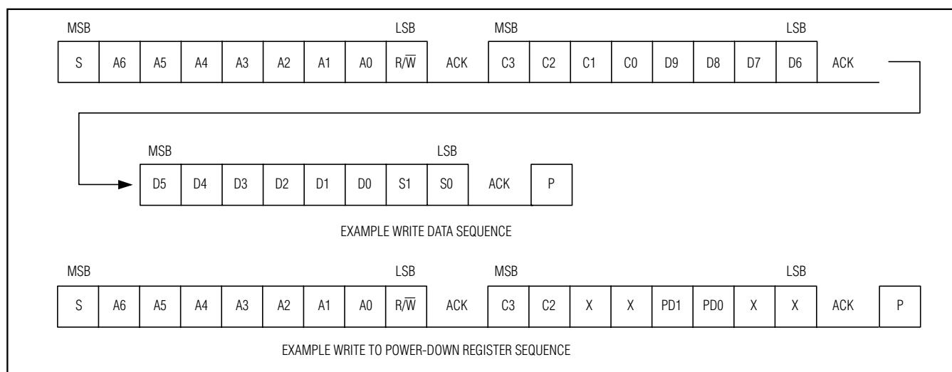
Figure 6. Example Write Command Sequences
