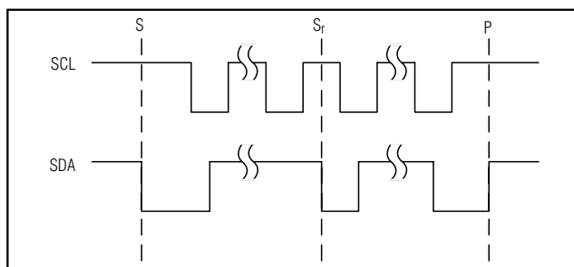
Figure 2. START/STOP Conditions
