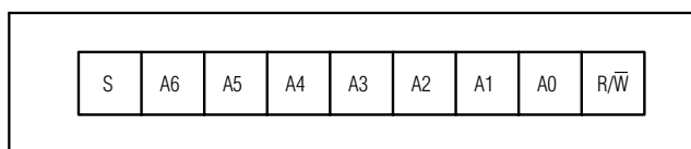
Figure 4. Slave Address Byte Definition
