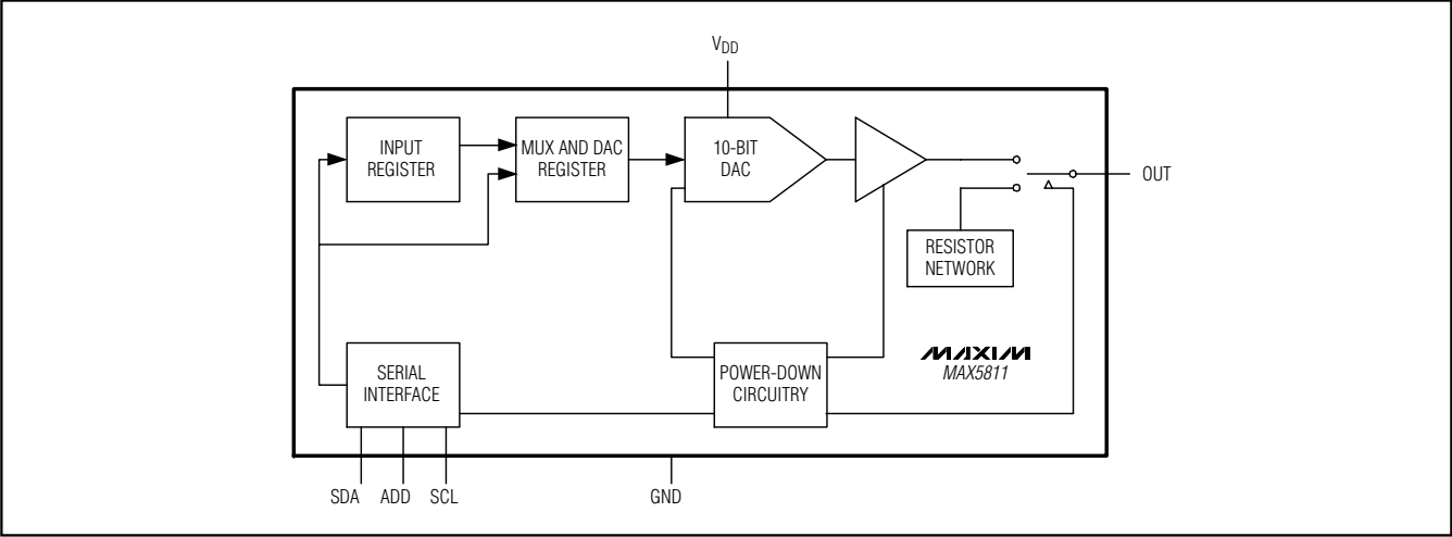
Functional Diagram
