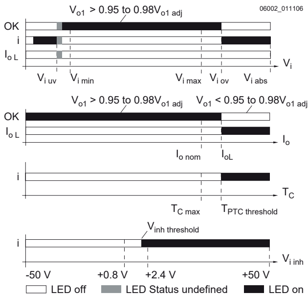
Fig. 18 LED indicators
