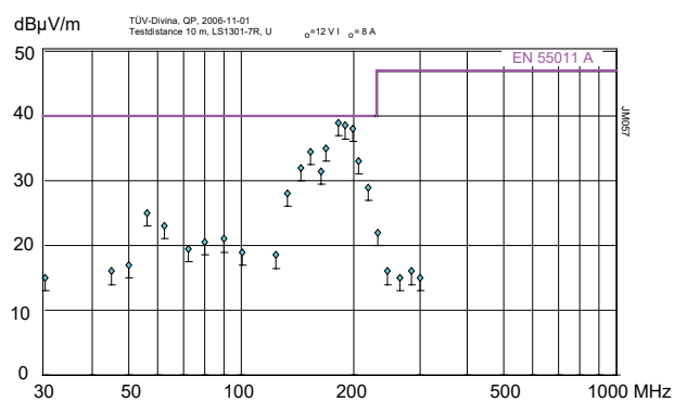
Fig. 22b Radiated emissions according to EN 55011/32, antenna 10 m distance, measured at V_{inom} and I_{onom} (LS1301-7R)
