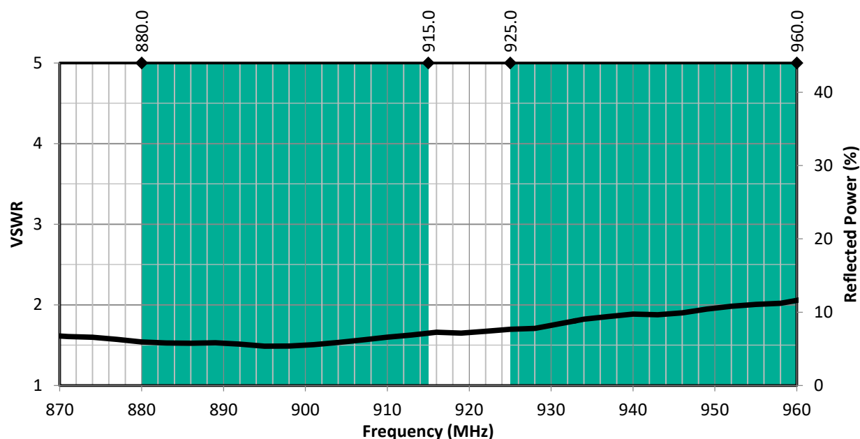
Figure 1. PW LTE Band 8 Antenna VSWR with Band 8 Uplink/Downlink Highlights
