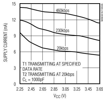
MAX3318/MAX3319 SUPPLY CURRENT vs. SUPPLY VOLTAGE
