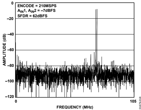
Figure 18. Two Tone Test A IN1 = 80.3 MHz, A IN2 = 81.3 MHz
