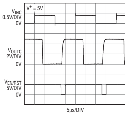
LT6108-1 Comparator Step Response (5mV INC Overdrive)
