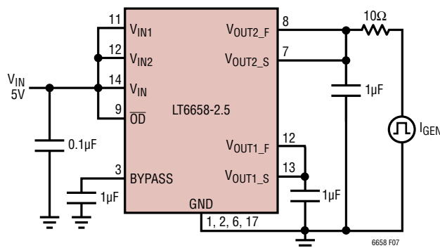
Figure 7. Load Current Response Time Test Circuit
