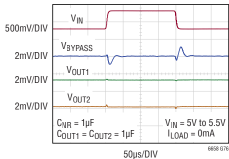
2.5V Line Transient Response
