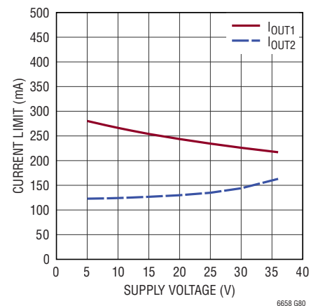
Current Limit vs Supply Voltage
