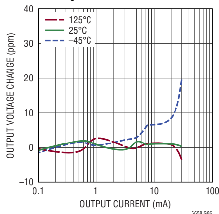
5V V_{OUT1} Load Regulation, Sinking
