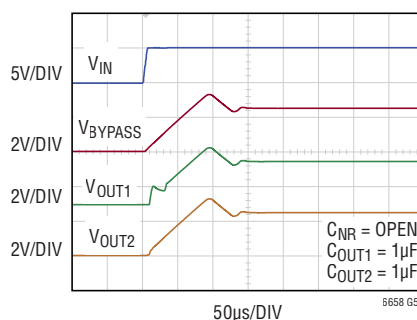
2.5V Turn-On Characteristic
