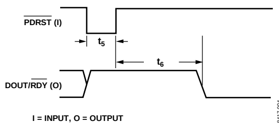
Figure 4. Resetting the AD7171
