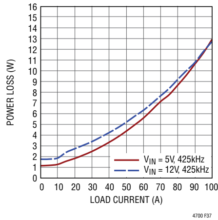
Figure 37. 1.2V Power Loss Curve
