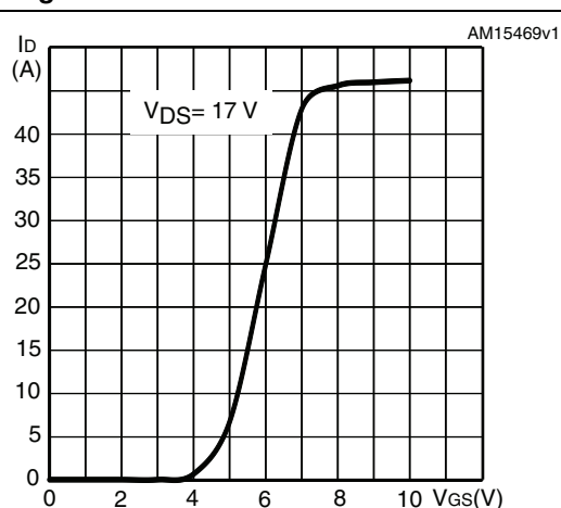
Figure 7. Transfer characteristics
