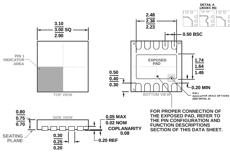
Figure 71. 10-Lead Lead Frame Chip Scale Package [LFCSP] 3 mm x 3 mm Body and 0.75 mm Package Height (CP-10-9)
