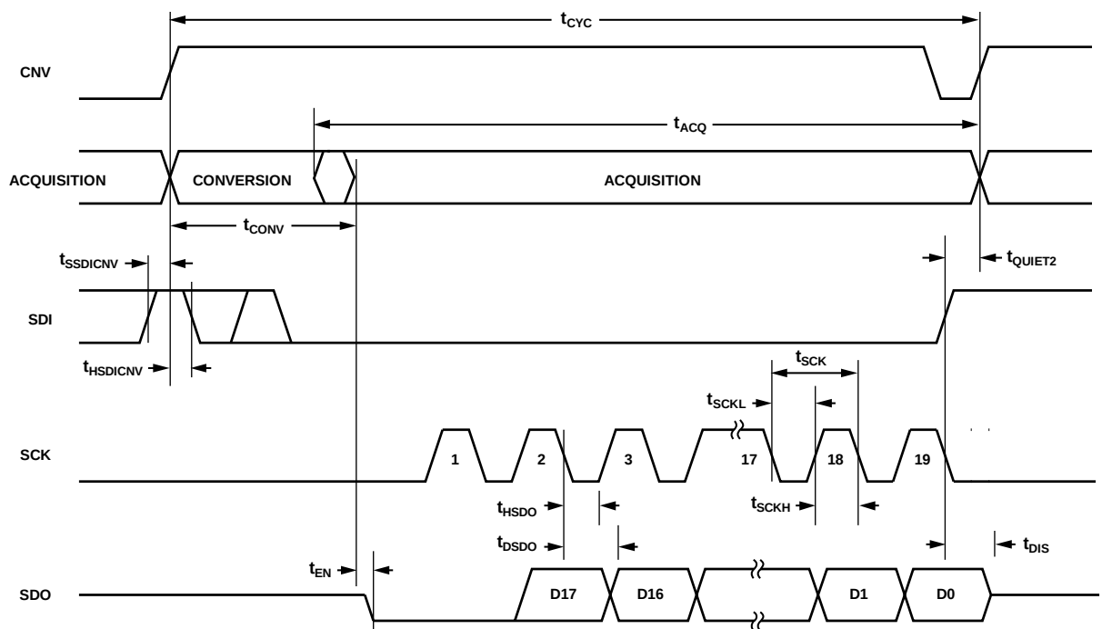
Figure 65. \overline{CS} Mode, 4-Wire with Busy Indicator Serial Interface Timing Diagram
