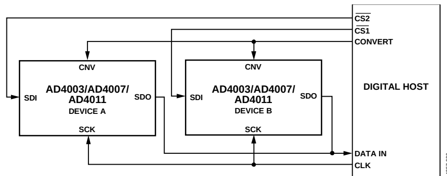
Figure 62. \overline{CS} Mode, 4-Wire Without Busy Indicator Connection Diagram
