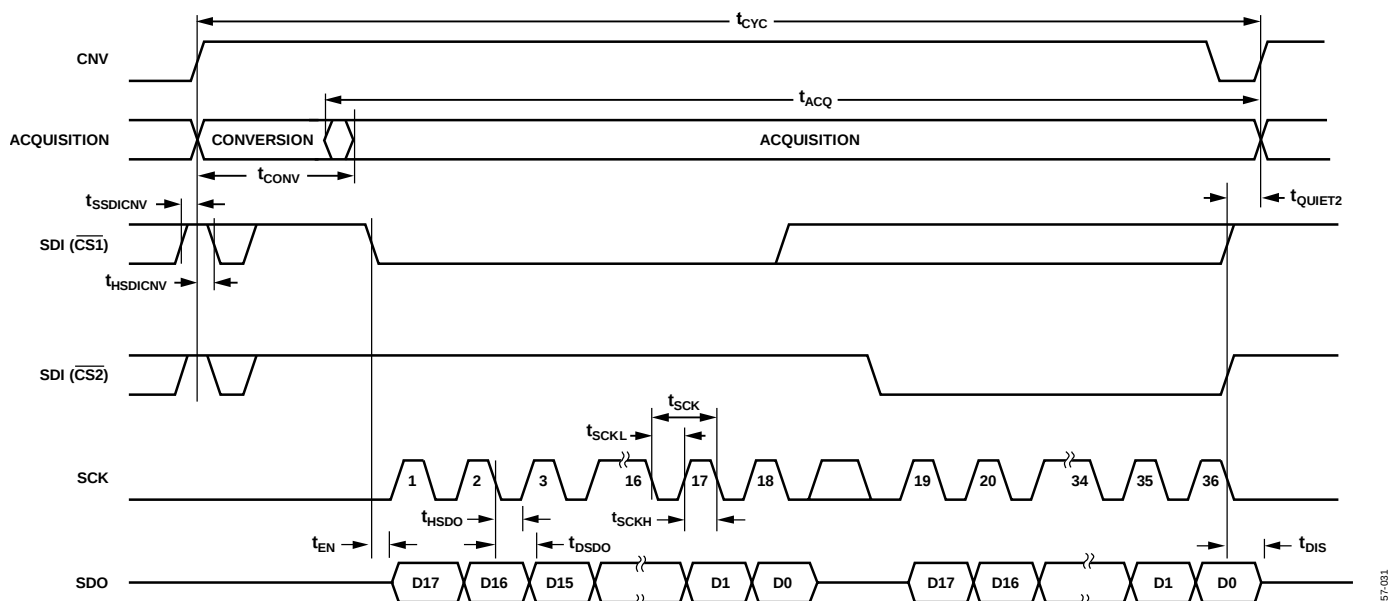
Figure 63. \overline{CS} Mode, 4-Wire Without Busy Indicator Serial Interface Timing Diagram
