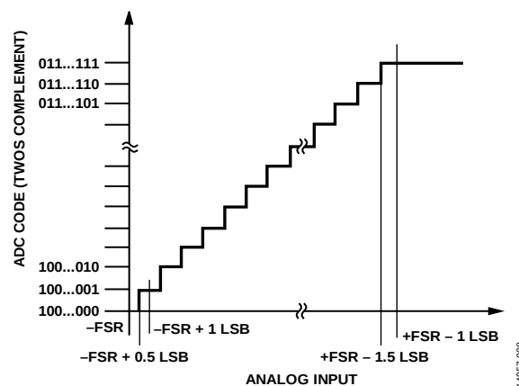
Figure 33. ADC Ideal Transfer Function (FSR Is Full-Scale Range)
