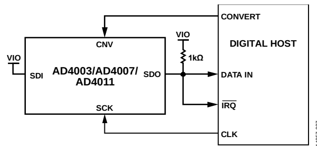
Figure 58. \overline{\text{CS}} Mode, 3-Wire with Busy Indicator Connection Diagram (SDI High)
