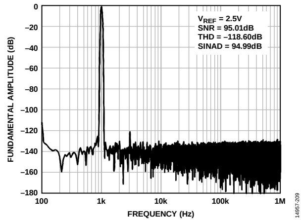
Figure 16. 1 kHz, -0.5 dBFS Input Tone FFT, Wide View, V_{REF} = 2.5\text{ V}
