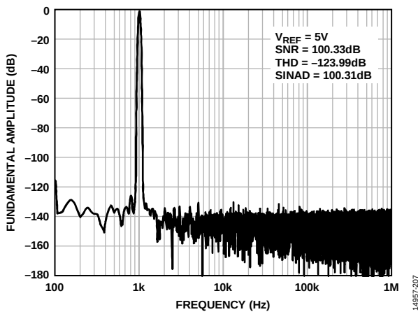
Figure 13. 1 kHz, -0.5 dBFS Input Tone Fast Fourier Transform (FFT), Wide View, V_{REF} = 5\text{ V}
