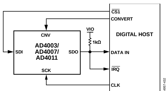
Figure 60. \overline{\text{CS}} Mode, 4-Wire Turbo Mode Connection Diagram
