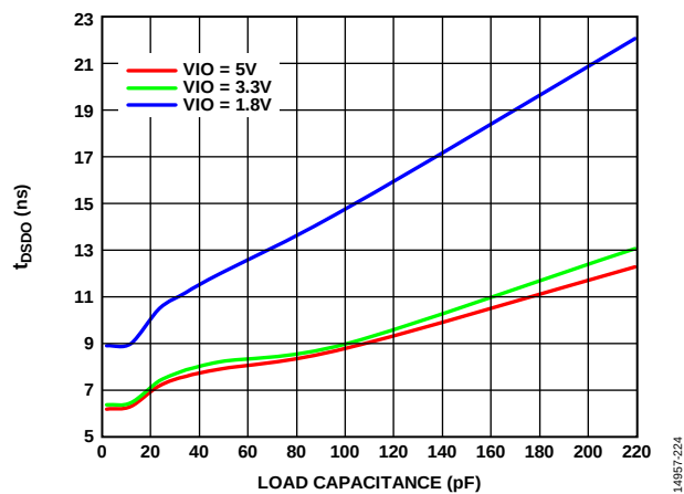
Figure 31. t BSDO vs. Load Capacitance
