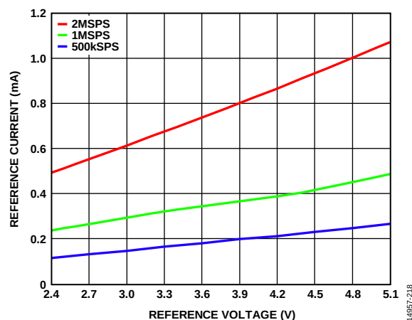
Figure 29. Reference Current vs. Reference Voltages
