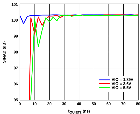
Figure 23. SINAD vs. t_{QUIET2}
