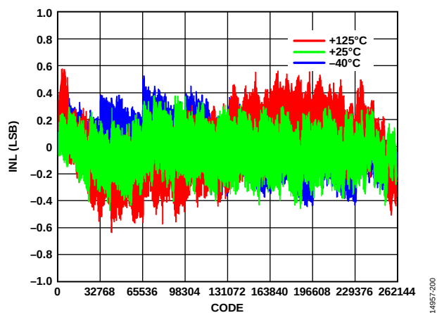
Figure 6. INL vs. Code for Various Temperatures, V_{REF} = 5\text{ V}
