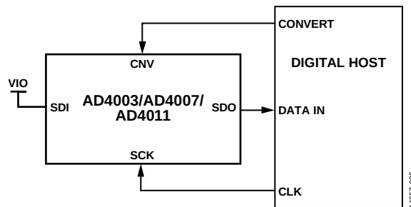
Figure 56. \overline{\text{CS}} Mode, 3-Wire Without Busy Indicator Connection Diagram (SDI High)
