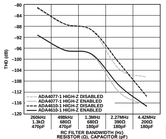
Figure 47. THD vs. RC Filter Bandwidths for Various Precision ADC Drivers, f_{IN} = 1 kHz (Turbo Mode On, High-Z Enabled/Disabled) V_{DD} = 1.8 V, V_{IO} = 3.3 V, V_{REF} = 5 V, 25^{\circ}\text{C}
