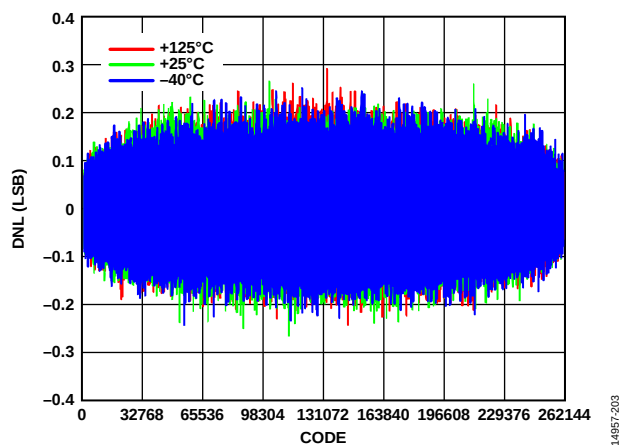
Figure 9. DNL vs. Code for Various Temperatures, V_{REF} = 5\text{ V}
