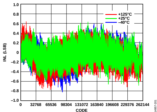
Figure 7. INL vs. Code for Various Temperatures, V_{REF} = 2.5\text{ V}
