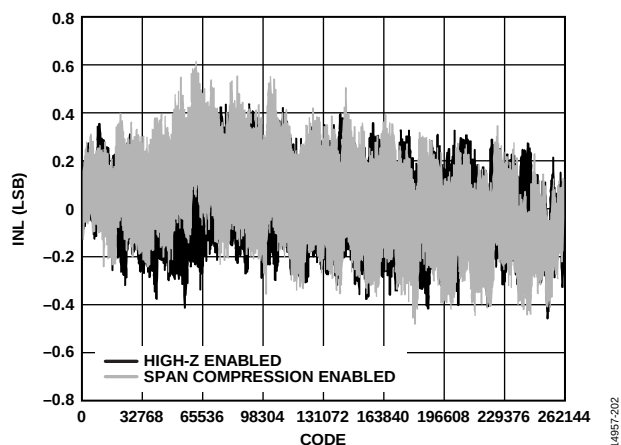
Figure 8. INL vs. Code, High-Z and Span Compression Modes Enabled, V_{REF} = 5\text{ V}
