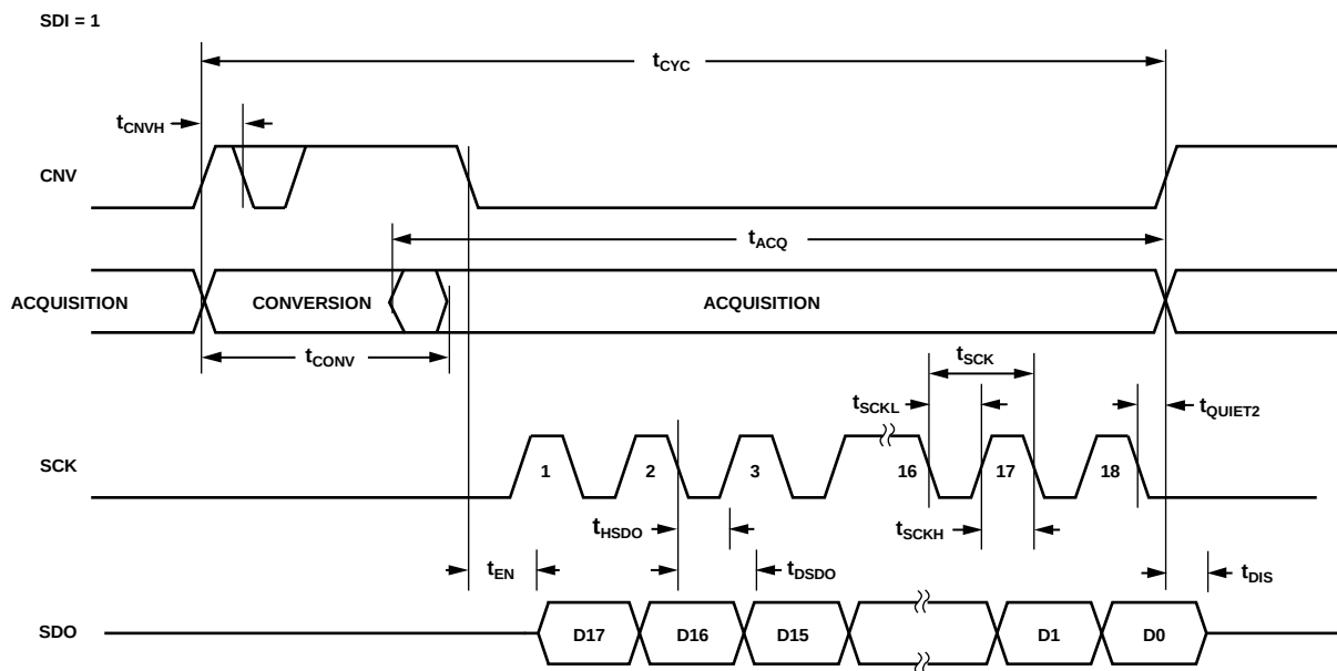
Figure 57. \overline{\text{CS}} Mode, 3-Wire Without Busy Indicator Serial Interface Timing Diagram (SDI High)
