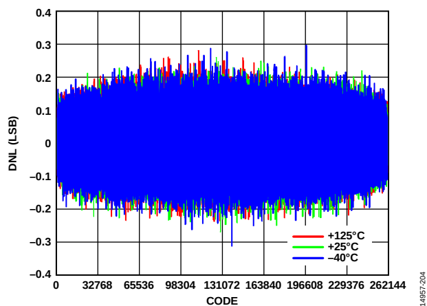
Figure 10. DNL vs. Code for Various Temperatures, V_{REF} = 2.5\text{ V}
