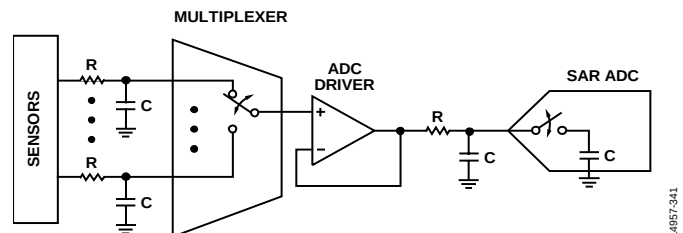
Figure 42. Multiplexed Data Acquisition Signal Chain Using the AD4003/AD4007/AD4011
