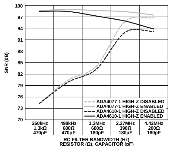
Figure 46. SNR vs. RC Filter Bandwidths for Various Precision ADC Drivers, f_{IN} = 1 kHz (Turbo Mode On, High-Z Enabled/Disabled), V_{DD} = 1.8 V, V_{IO} = 3.3 V, V_{REF} = 5 V, 25^{\circ}\text{C}
