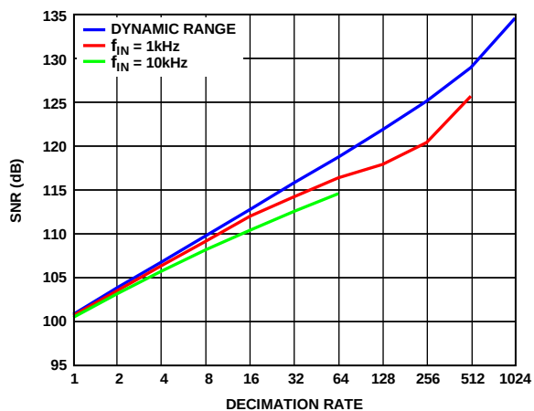
Figure 20. SNR vs. Decimation Rate for Various Input Frequencies, 2 MSPS
