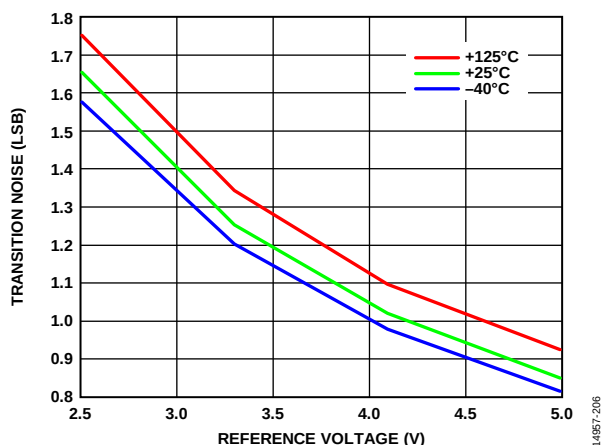
Figure 11. Transition Noise vs. Reference Voltage for Various Temperatures
