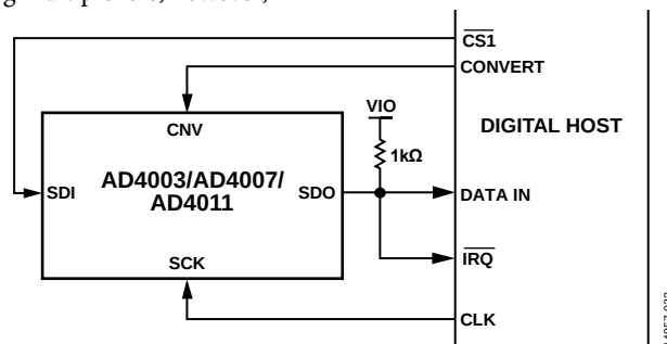
Figure 64. \overline{\text{CS}} Mode, 4-Wire with Busy Indicator Connection Diagram
