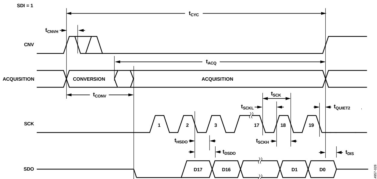
Figure 59. \overline{\text{CS}} Mode, 3-Wire with Busy Indicator Serial Interface Timing Diagram (SDI High)
