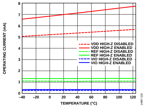
Figure 25. Operating Current vs. Temperature, AD4003, 2 MSPS
