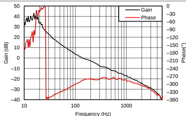
Figure 62. Measured Control Loop Gain/Phase at 300 V DC , Light Load 0.2 A
