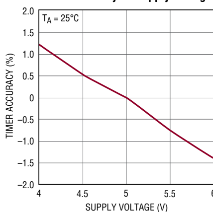
Timer Accuracy vs Supply Voltage
