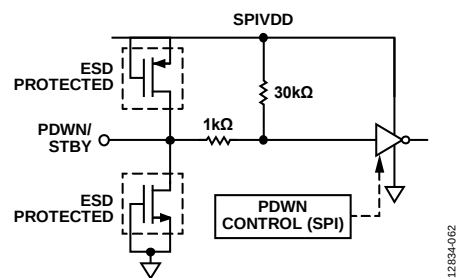
Figure 62. PDWN/STBY Input
