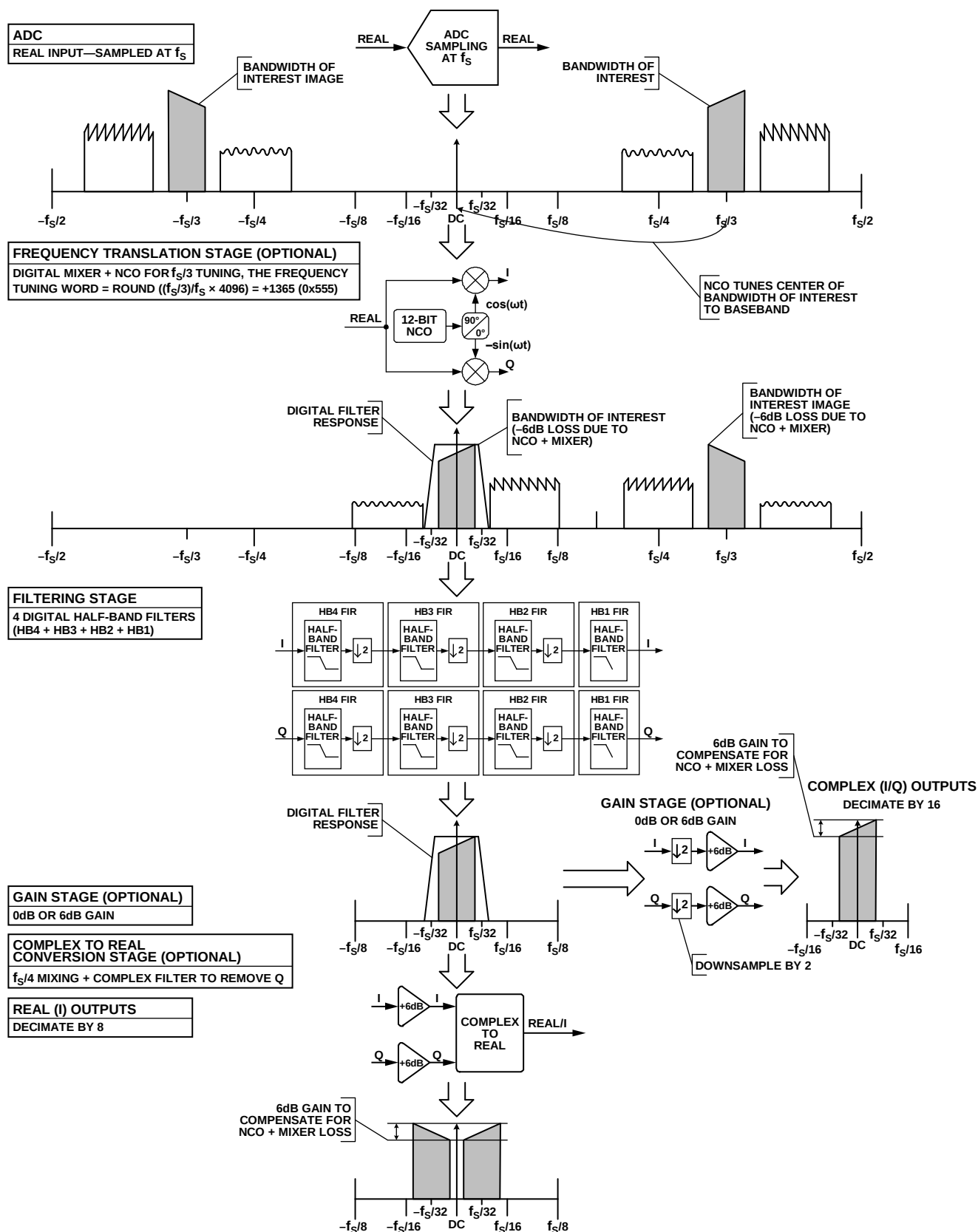
Figure 89. DDC Theory of Operation Example (Real Input—Decimate by 16)
