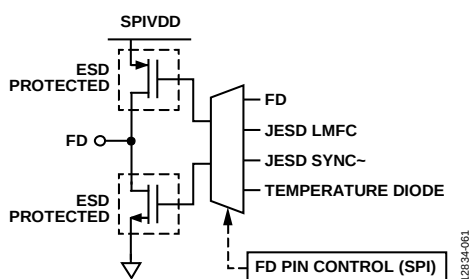
Figure 61. FD Outputs
