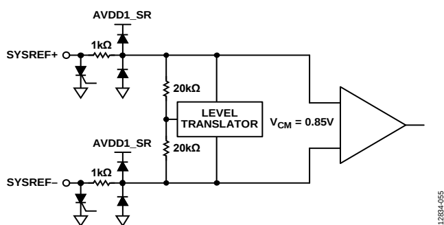
Figure 55. SYSREF± Inputs
