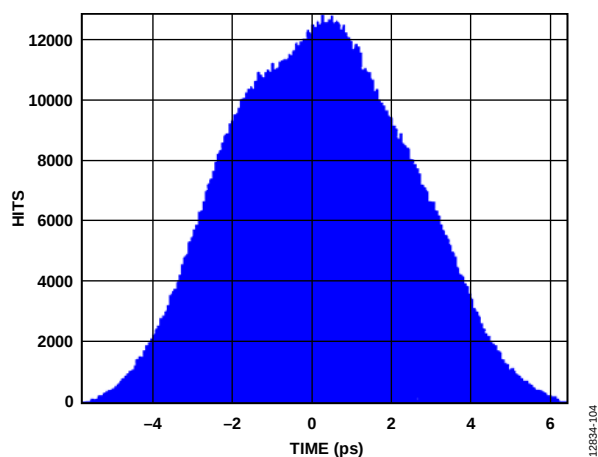
Figure 104. Digital Outputs Histogram, External 100 \Omega Terminations at 10 Gbps
