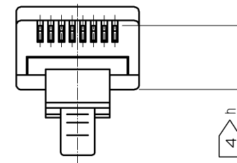
ASSEMBLED DIAGRAM (2 : 1)
