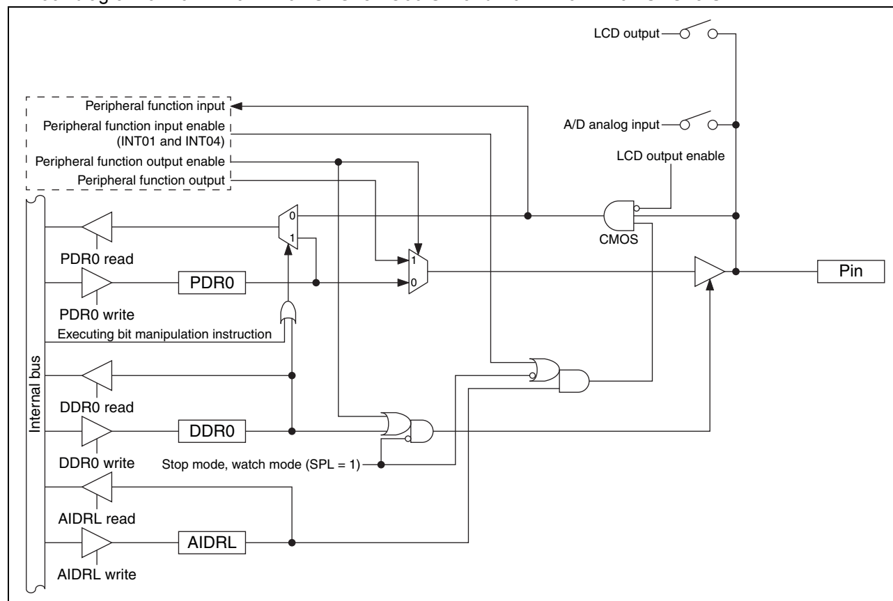
• Block diagram of P01/INT01/AN01/SEG28/TO00/UI2 and P04/INT04/AN04/SEG25/UI1
