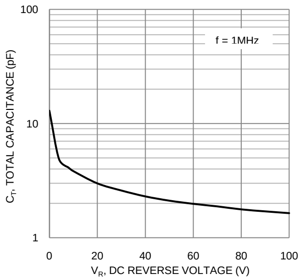
Figure 5. Total Capacitance
