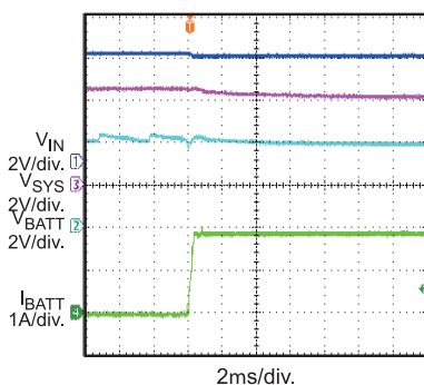
Battery Insertion
