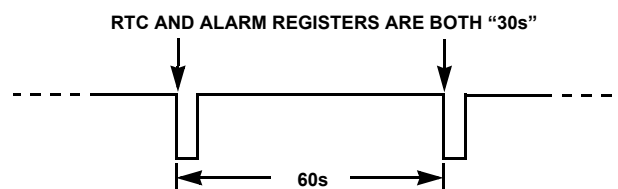
FIGURE 15. \overline{\text{IRQ}}/\text{FOUT} WAVEFORM
