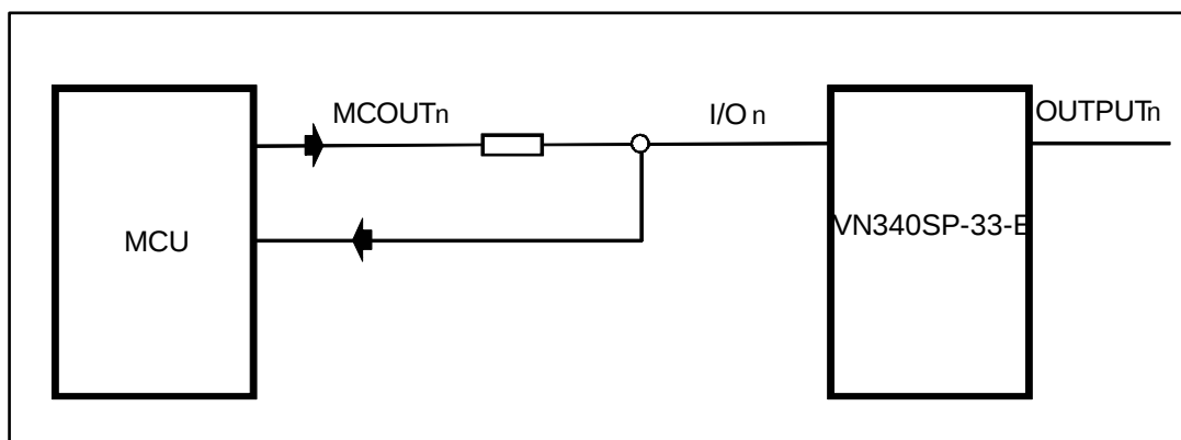
Figure 9: Driving circuit
