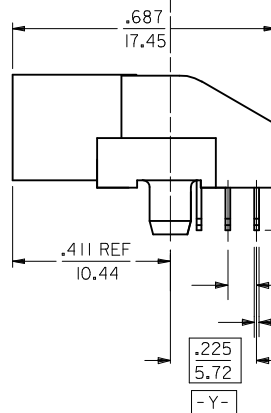
END DETAIL OPTION A (BOTH ENDS)
