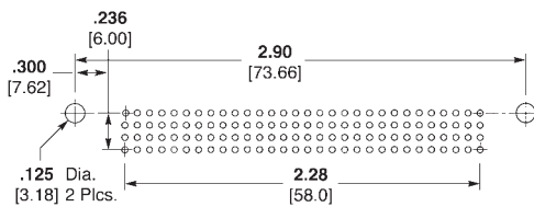
Recommended PC Board Layout for 1375965-4
