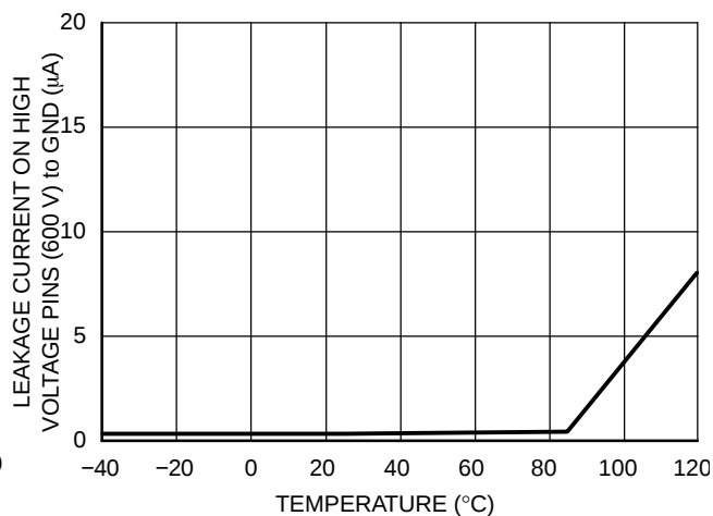
Figure 40. Leakage Current on High Voltage Pins (600 V) to Ground vs. Temperature ( V_{BRIDGE} = V_{BOOT} = V_{DRV\_HI} = 600 V)
