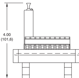
DIN-Rail Mount
