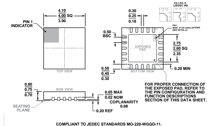
Figure 54. 20-Lead Lead Frame Chip Scale Package [LFCSP] 4 mm × 4 mm Body and 0.75 mm Package Height (CP-20-8) Dimensions shown in millimeters
