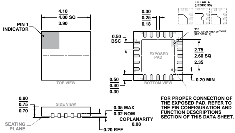
COMPLIANT TO JEDEC STANDARDS MO-220-WGGD-11. Figure 54. 20-Lead Lead Frame Chip Scale Package [LFCSPP] (CP-20-8) 4 mm x 4 mm Body and 0.75 mm Package Height Dimensions shown in millimeters
