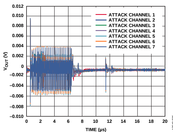
Figure 34. DAC-to-DAC Crosstalk
