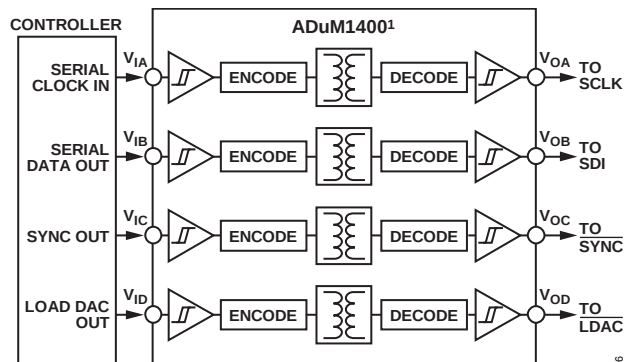
Figure 52. Isolated Interface
