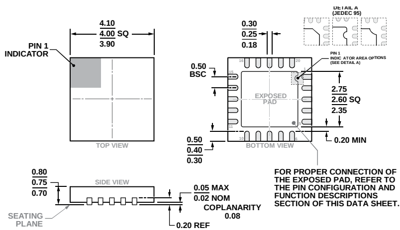
Figure 54. 20-Lead Lead Frame Chip Scale Package [LFCSP] 4 mm × 4 mm Body and 0.75 mm Package Height (CP-20-8)
