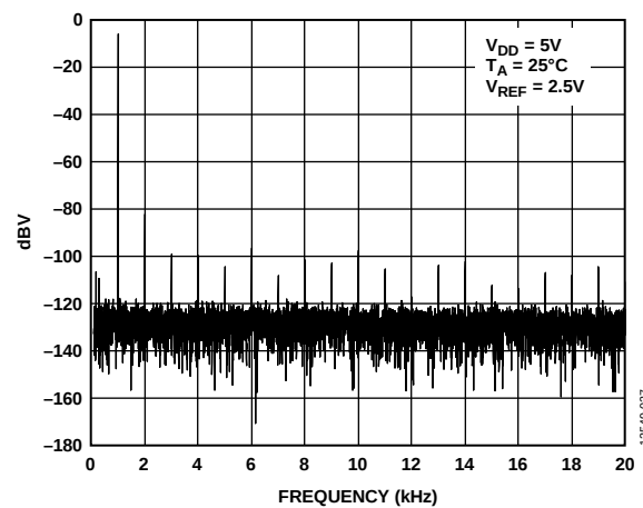
Figure 37. THD at 1 kHz
