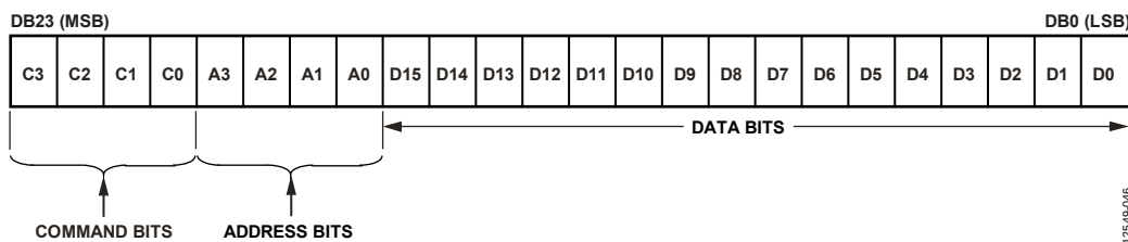
Figure 44. Input Shift Register Content
