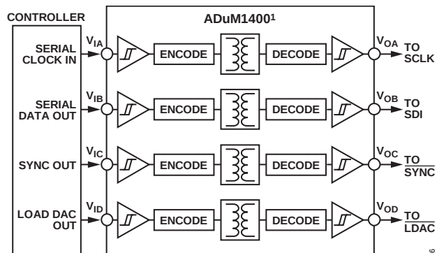
Figure 52. Isolated Interface
