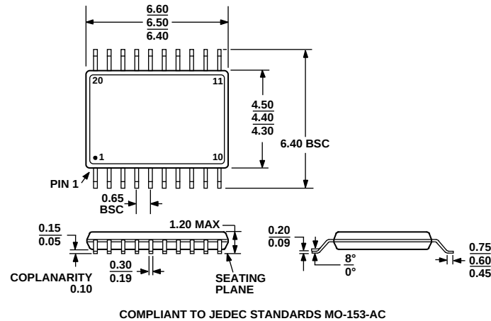
Figure 53. 20-Lead Thin Shrink Small Outline Package [TSSOP] (RU-20) Dimensions shown in millimeters
