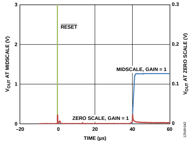
Figure 40. Hardware Reset
