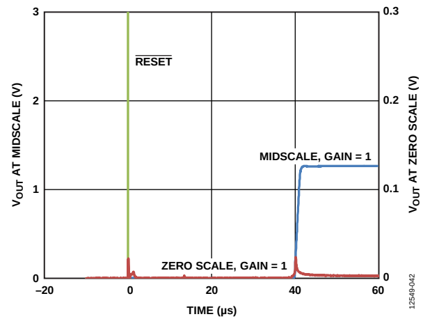
Figure 40. Hardware Reset
