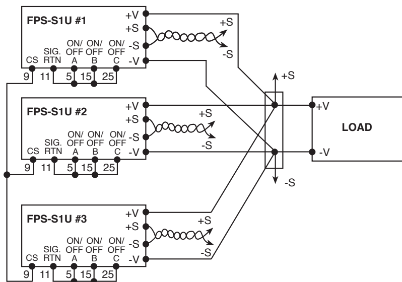
Fig 13-2: Parallel operation with Remote sensing
