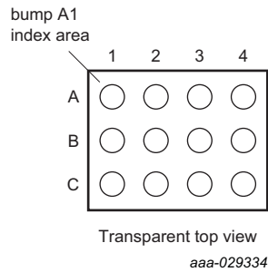
Fig 5. Pin configuration for WLCSP12
