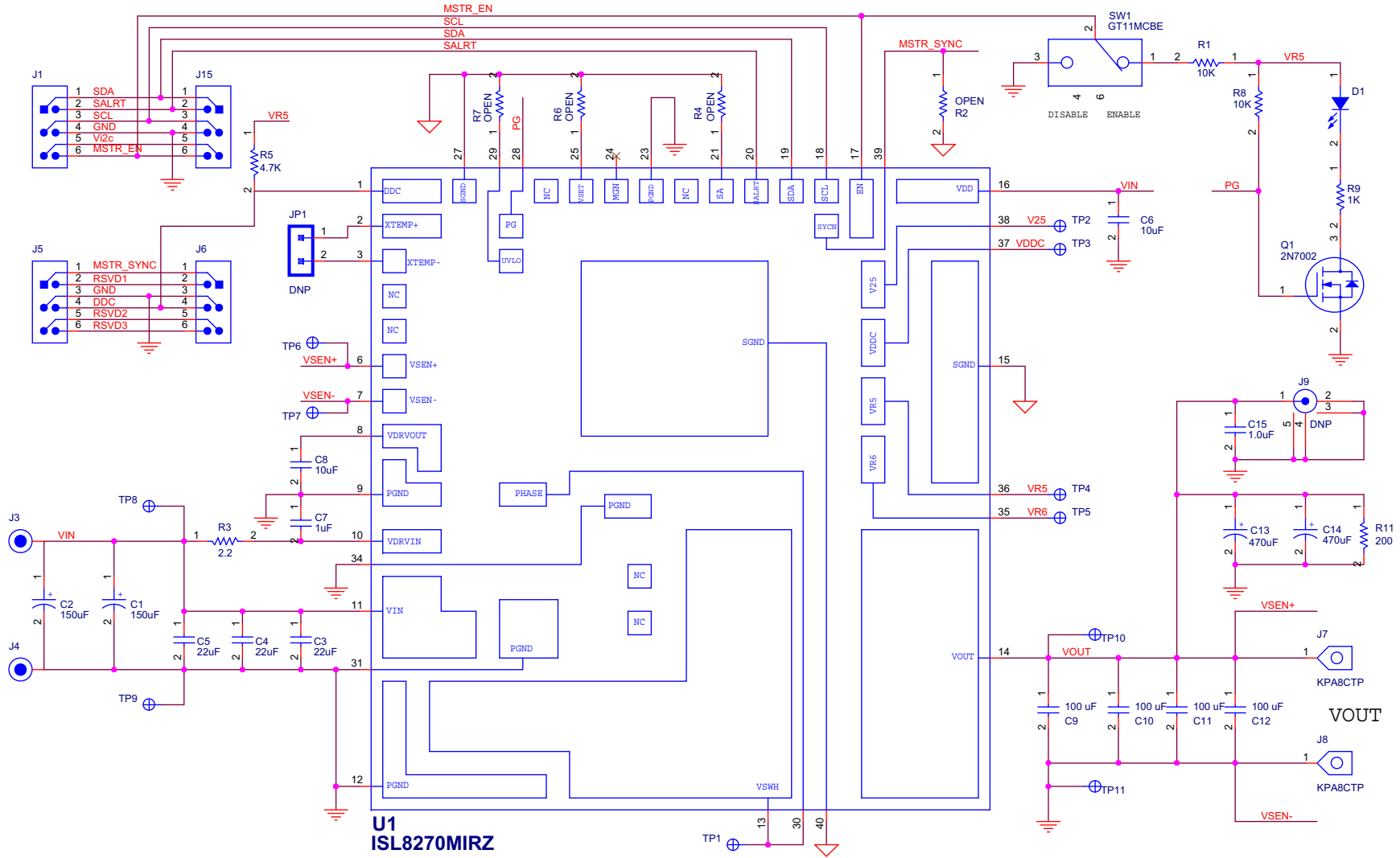
FIGURE 2. APPLICATION CIRCUIT
