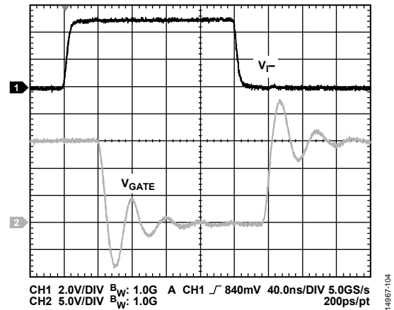
Figure 7. V_{I-} to V_{GATE} Waveform for 2 nF Load, 0 Ω Series Gate Resistor, V_{DD2} = 15 V
