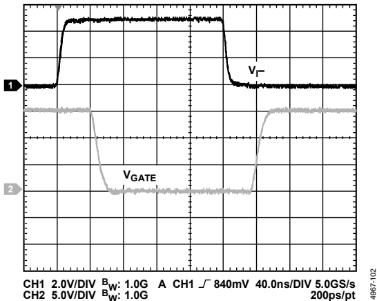
Figure 5. V_{I-} to V_{GATE} Waveform for 2 nF Load, 3.9 \Omega Series Gate Resistor, V_{DD2} = 15 V
