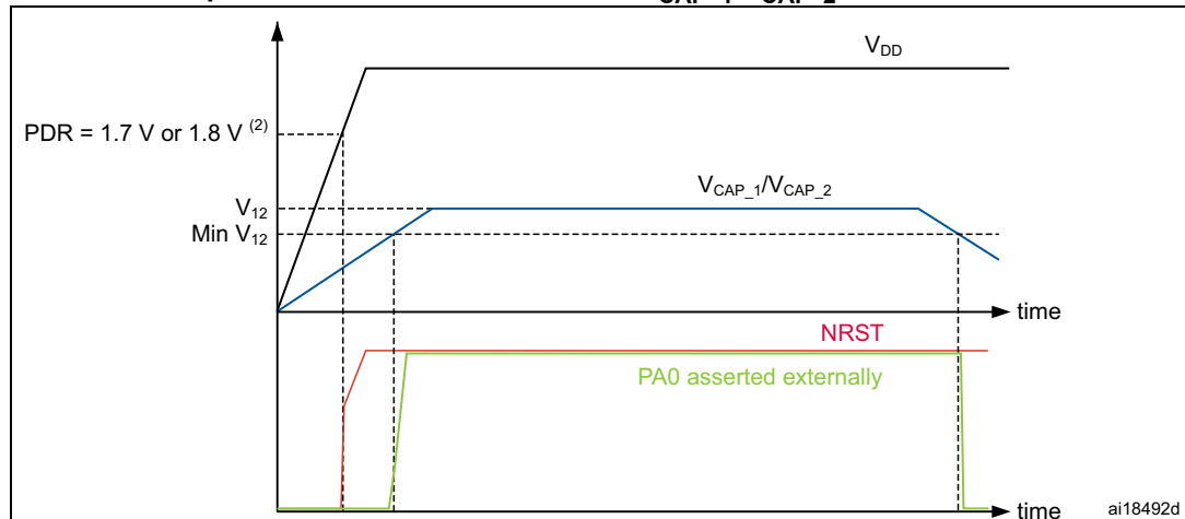
Figure 11. Startup in regulator OFF mode: fast V_{DD} slope - power-down reset risen before V_{CAP\_1}/V_{CAP\_2} stabilization
