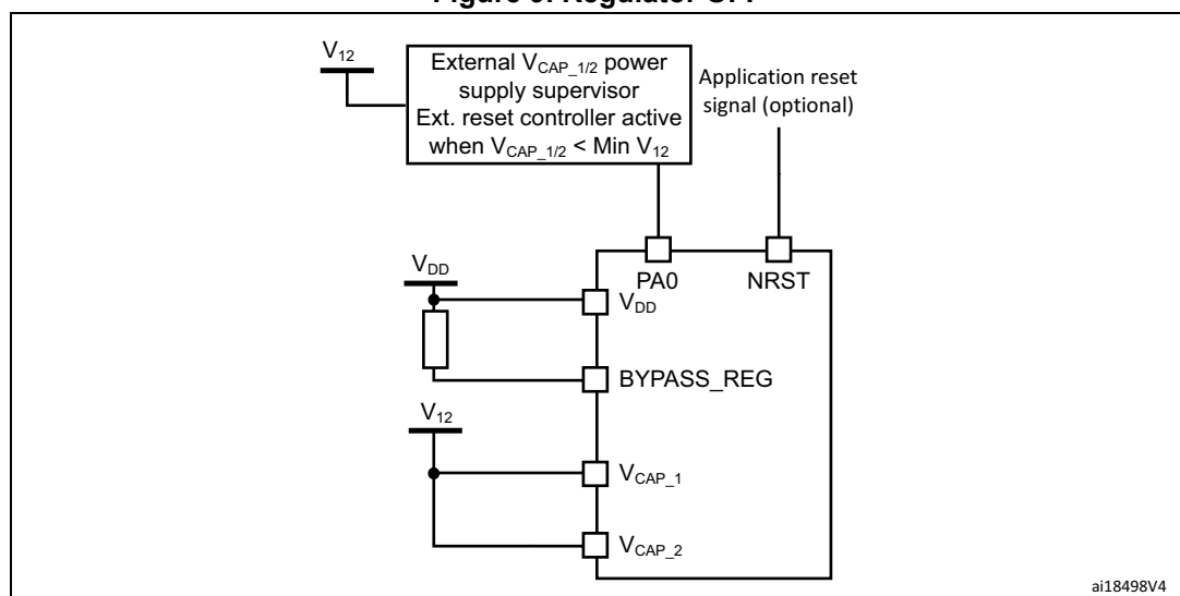
Figure 9. Regulator OFF
