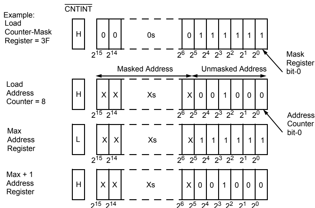
Figure 3. Programmable Counter-Mask Register Operation 17/
