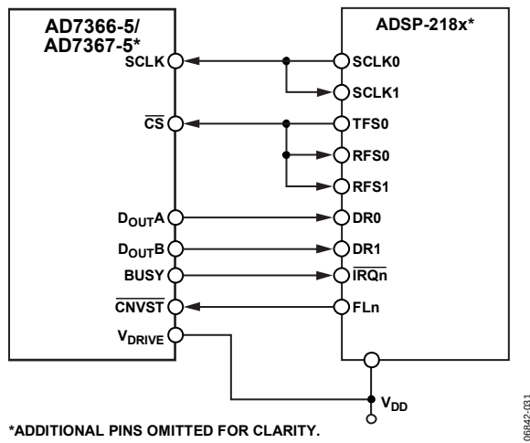
Figure 29. Interfacing the AD7366-5/AD7367-5 to the ADSP-218x
