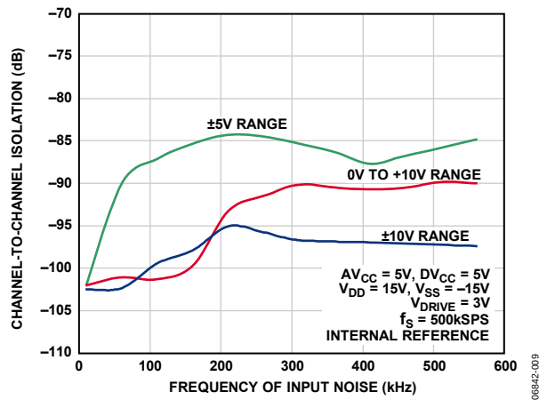
Figure 9. Channel-to-Channel Isolation
