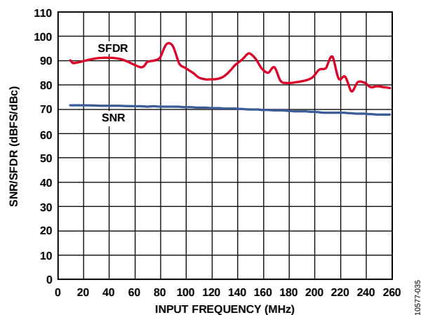
Figure 35. SNR/SFDR vs. f_{IN} ; f_{SAMPLE} = 125 MSPS
