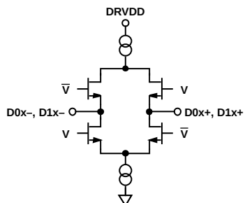
Figure 46. Equivalent Digital Output Circuit
