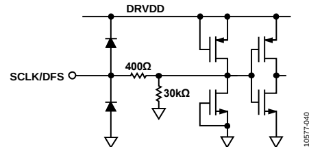
Figure 47. Equivalent SCLK/DFS Input Circuit
