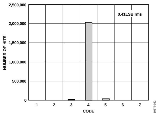
Figure 22. Input Referred Noise Histogram; f_{SAMPLE} = 80 MSPS
