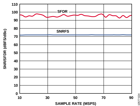
Figure 24. SNR/SFDR vs. Sample Rate; f_{IN} = 9.7 MHz, f_{SAMPLE} = 80 MSPS
