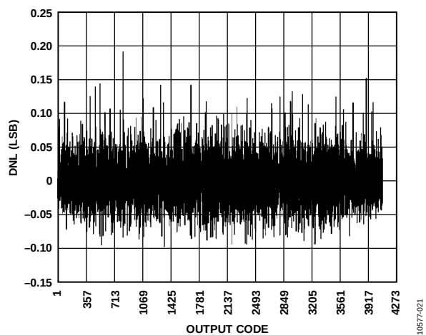
Figure 21. DNL; f_{IN} = 9.7 MHz, f_{SAMPLE} = 80 MSPS
