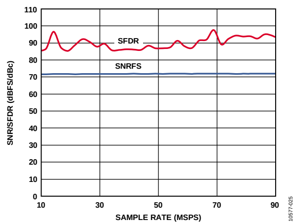
Figure 25. SNR/SFDR vs. Sample Rate; f_{IN} = 70 MHz, f_{SAMPLE} = 80 MSPS
