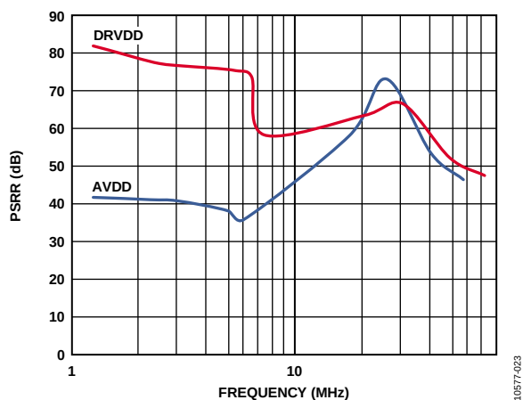
Figure 23. PSRR vs. Frequency; f_{CLK} = 125 MHz, f_{SAMPLE} = 80 MSPS
